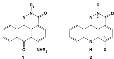
Figure 1. The structures of anthrapyridazones ( 1 ) and pyridazoacridines ( 2 ).
