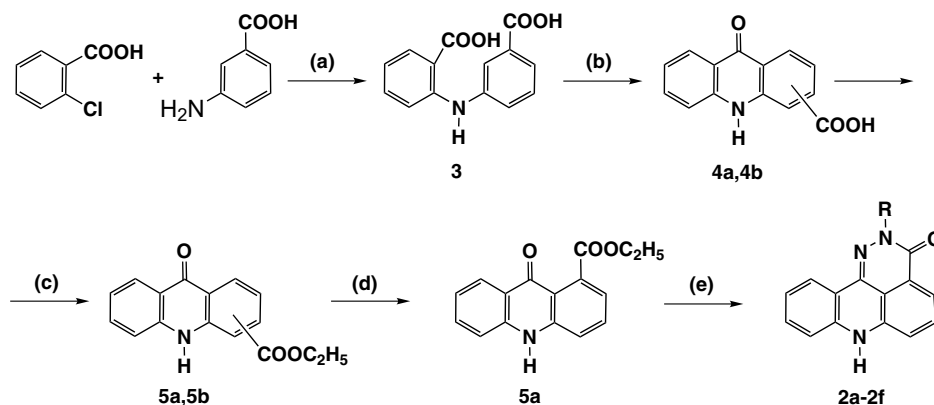
Scheme 1. Synthetic route for compounds 2a–f . Reagents and conditions: (a) Cu powder, K 2 CO 3 , i -C 3 H 11 OH, reflux/3 h; (b) concd H 2 SO 4 , 100 °C/1 h; (c) EtOH/dry HCl, reflux/4 h; (d) chromatography on silica gel; (e) for 2a : NH 2 NH 2 ·xH 2 O, 125 °C/6 h; for 2b–f : 1. POCl 3 , 125 °C/1 h; 2. NH 2 NHR, 125 °C/2.5–3 h.
