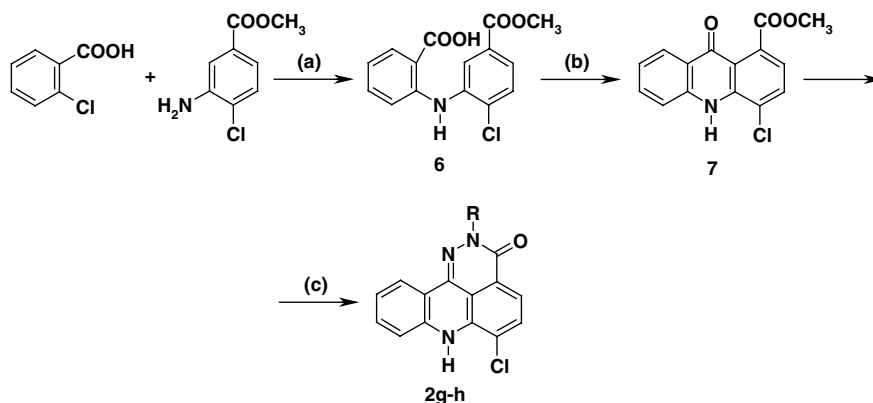
Scheme 2. Synthetic route for compounds 2g–h . Reagents and conditions: (a) N -methylpyrrolidinone and N,N -diisopropylethylamine, Cu(OAc) 2 ·xH 2 O, 130 °C/3 h; (b) PPE, 100 °C/1 h; (c) for 2g : 1. POCl 3 , reflux/0.5 h, 2. NH 2 NH(CH 2 ) 3 N(CH 3 ) 2 , DMA, 130 °C/3 h; for 2h : NH 2 NH 2 ·xH 2 O, DMA, 125 °C/2 h.
